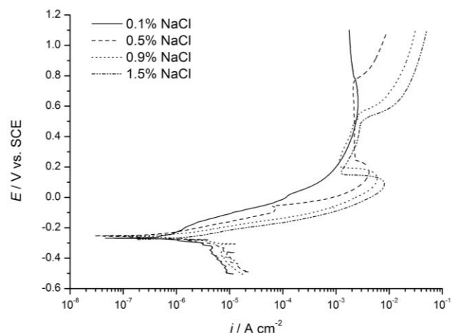
Figure 5 Potentiodynamic polarization curves for the CuAlNi alloy in NaCl solutions
