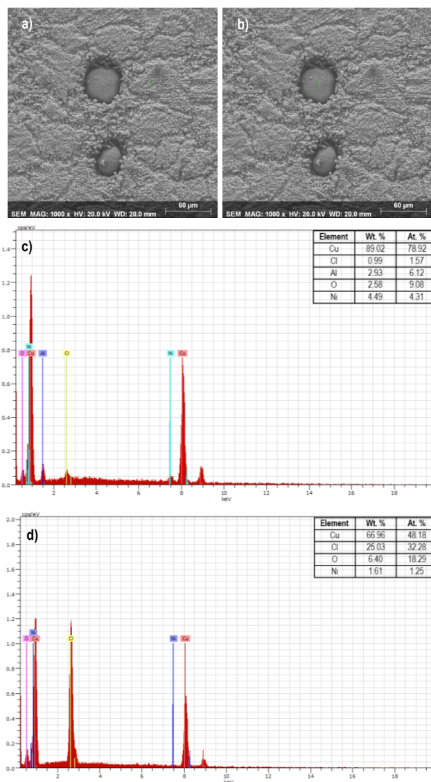
Figure 7 SEM micrograph with a marked position for the EDS analysis outside the pit a), inside the pit b), EDS results outside the pit c) and inside the pit d) for the CuAlNi alloy after the polarization measurements in the 0.9% NaCl solution
