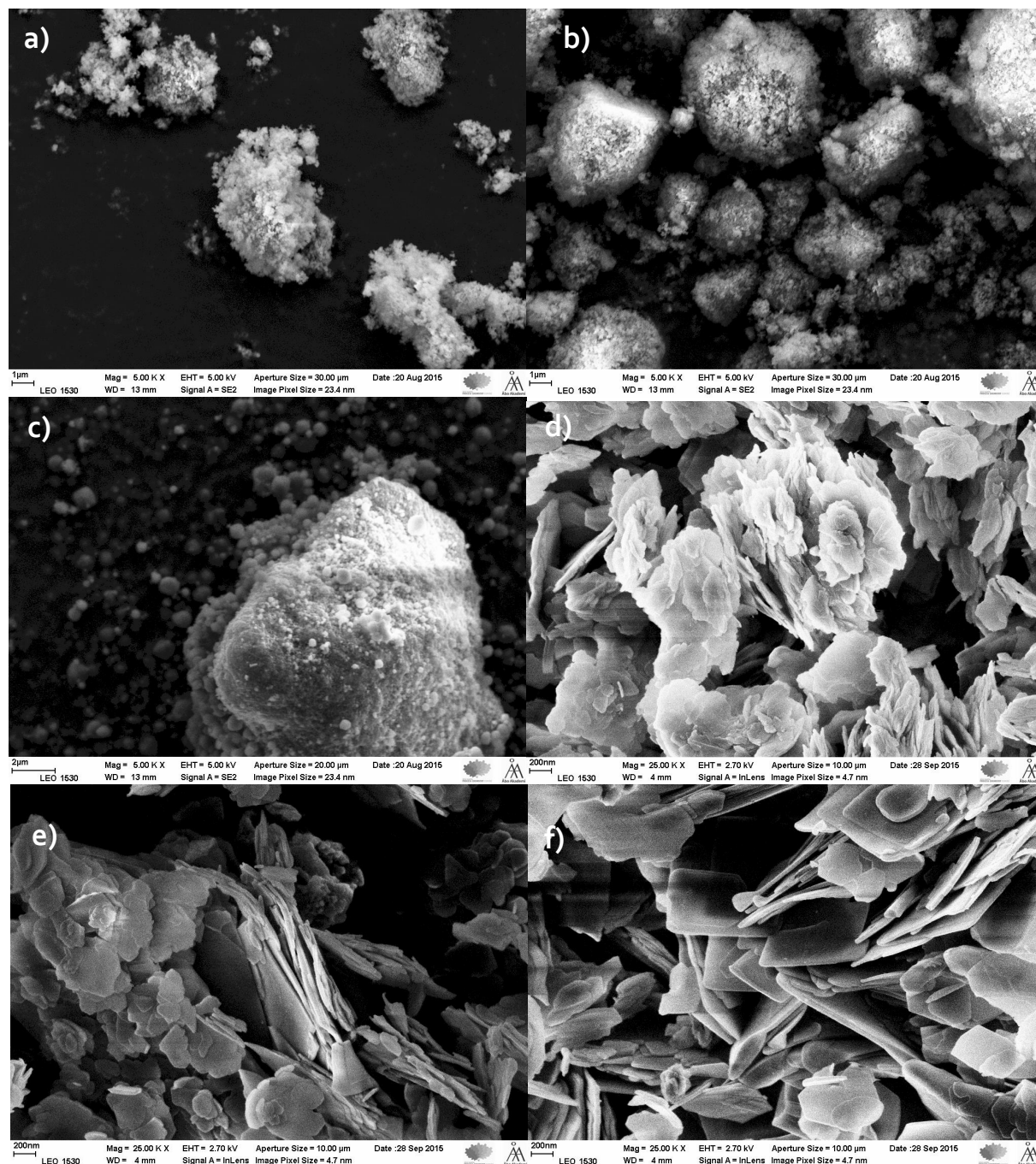
Figure 2 SEM images of Cu-BETA-25, Cu-BETA-150, Cu-BETA-300 (a-c) and Cu-MCM-22-30, Cu-CM-22-50, Cu-MCM-22-100 (d-f)
