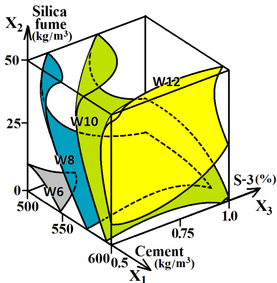
Figure 4 Effect of composition on the water resistance of expanded clay concrete.
