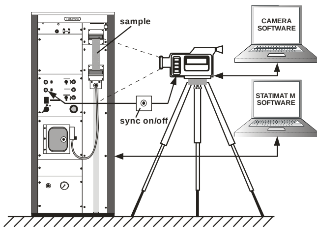
Figure 2 Schematic view of the experiment
