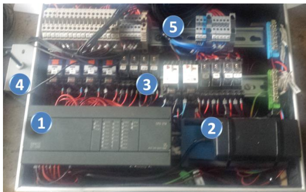
Figure 5. Simulation station
