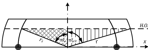
Figure 7 Incised section part with indicated radiuses and angles
