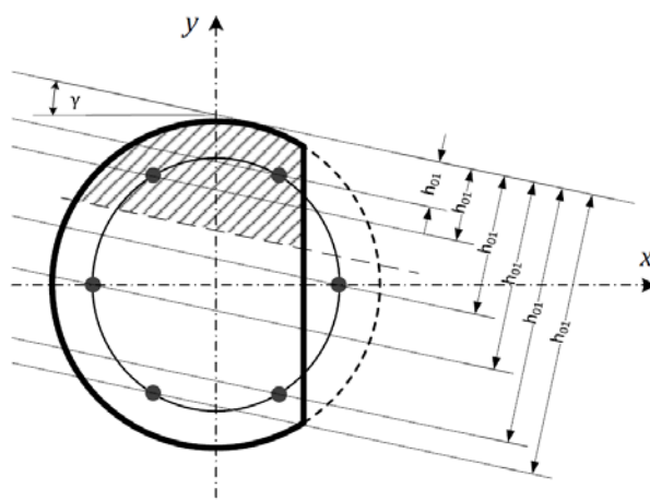
Figure 8 h_{0n} Distance from the compressive edge of element to the centroid of each reinforcement bar.
