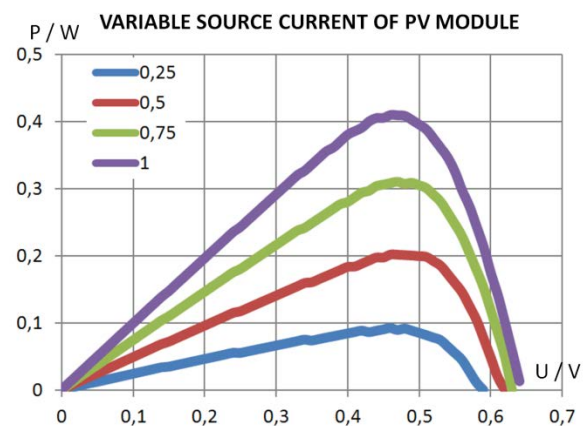
Figure 11. P-U characteristics for variable values of I_L and fixed R_p = 10 \Omega i R_s = 0.1 \Omega
