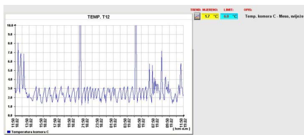
Figure 4. Temperature overview – fresh meat chamber
