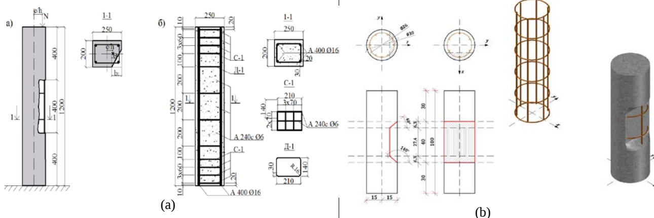
Figure 1 Scheme of column models (samples) with internal reinforcements and designed damage
